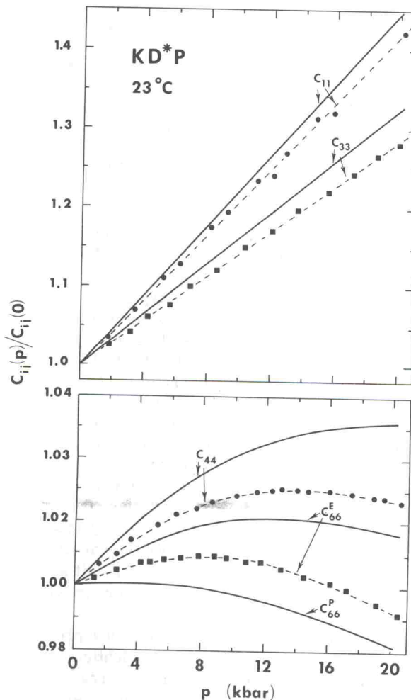
FIG. 2. Same as Fig. 1 for \text{KD}_2\text{PO}_4 (dKDP).
